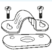
Spacer Bar Saddle No. KB 431 Material: Steel Finishes: Black Enamel, Galvanised Size: 20mm 25mm 32mm
