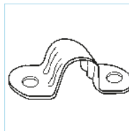
1Way (Single) Saddle No. KB 451 Material: Steel Finishes: Black Enamel, Galvanised Size: 20mm 25mm 32mm
