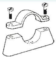
Hospital Saddle No. KB 362 Material: Malleable Iron Base, Steel Top Finishes: Black Enamel, Galvanised Size: 20mm 25mm
