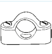
Distance Saddle No. KB 363 Material: Malleable Iron Base, Steel Top Finishes: Black Enamel, Galvanised Size: 20mm 25mm 32mm
